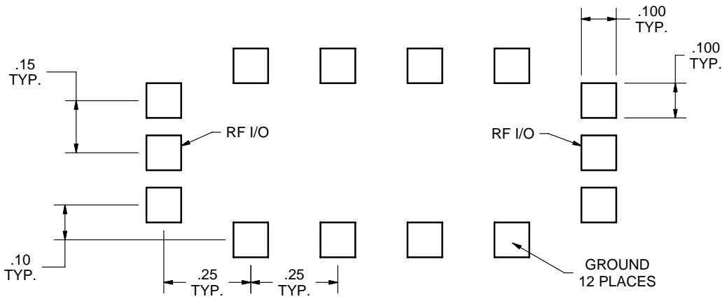
PRINTED CIRCUIT LAYOUT SCALE 4 : 1
